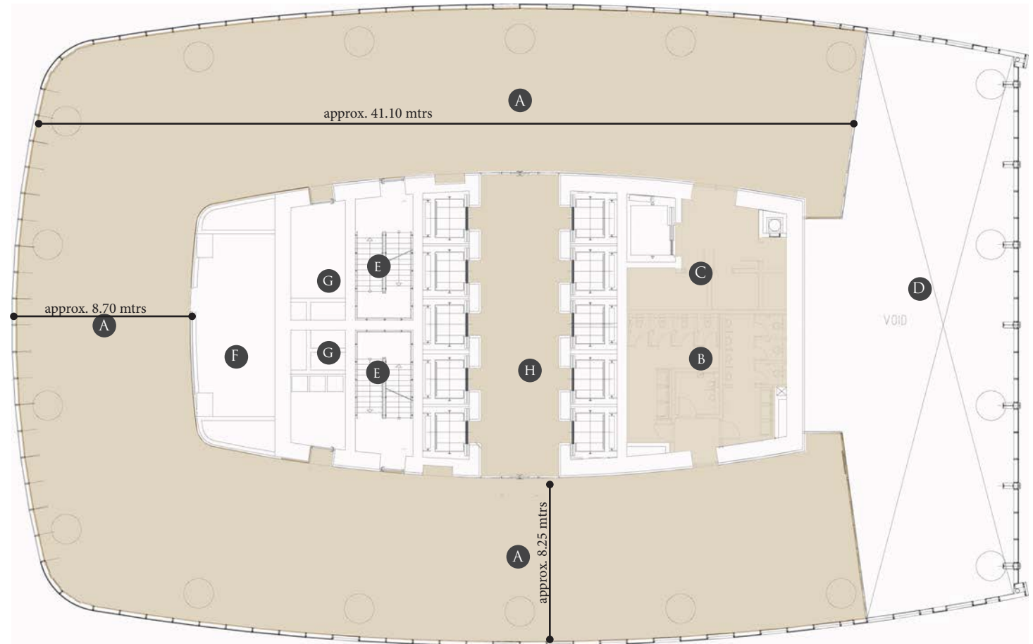
Winter Garden Floor Plan
